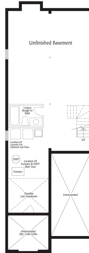
Basement Plan
